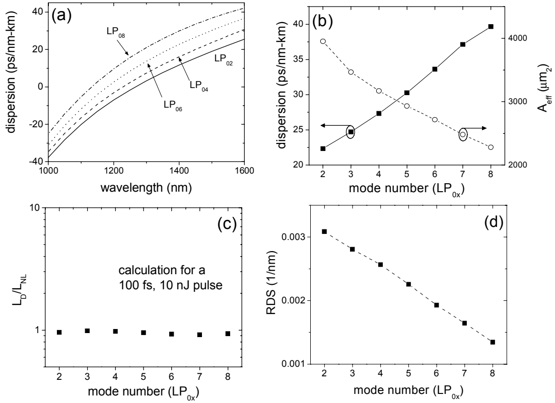
Figure 2 : Properties of the higher order modes. (a) Dispersion of several different higher-order-modes calculated from the measured index profile. (b) Dispersion and A_{eff} as a function of mode number at 1550 nm. (c) L_D/L_{NL} as a function of mode number for a 100 fs, 10 nJ pulse. (d) Relative Dispersion Slope (RDS) as a function of mode number at 1550 nm.
