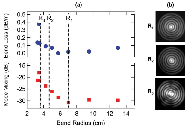
Fig. 4. (Color online) HOM propagation characterization in 3 m long fiber as shown in Fig. 3(c). (a) Excess bend loss (top) and mode-mixing efficiency (bottom) versus bend radius. (b) Near-field images for bend radii R_1=7 cm, R_2=4.5 cm, R_3=3.8 cm. There is no change for R > 7 cm; there are distortions for R < 4 cm. Modal output is stable down to R \sim 4.5 cm.
