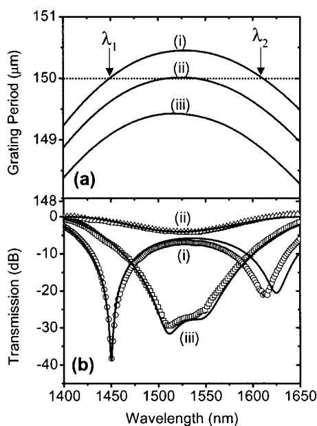
FIG. 1. (a) Simulated phase matching curves for a LPG that couples the fundamental core mode to the LP_{0,12} cladding mode immersed in fluids with different refractive indices (i) n = 1.41 , (ii) n = 1.39 , and (iii) n = 1.33 . For a grating with 150 \mu\text{m} period, the phase matching curves show resonance at two wavelengths (indicated by vertical arrows), turn around point (TAP), and no resonance for (i), (ii), and (iii), respectively. (b) corresponding simulated (solid curves) transmission spectra for the three fluids in (a). The symbols show the experimental transmission spectra for a grating with 150 \mu\text{m} period optimized to exhibit TAP in silicone oil ( n = 1.39 ). ( \Delta ), ( \square ), and ( \circ ) correspond to the case when the grating is immersed in water ( n = 1.33 ), silicone oil, and 41% sodium dichromate solution ( n = 1.41 ), respectively.
