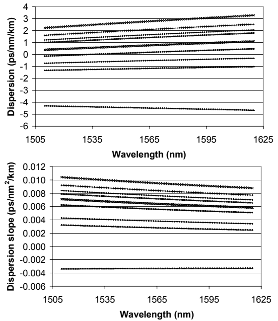
Figure 1 and 2. Measured dispersion of 9 DFF-HNLF fibers and calculated dispersion slope.
