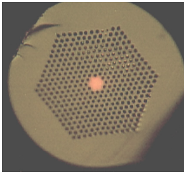
Figure 4. Photonic band gap fiber filled with high index oil.
