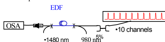
Figure 1 L-band amplifier configuration.
