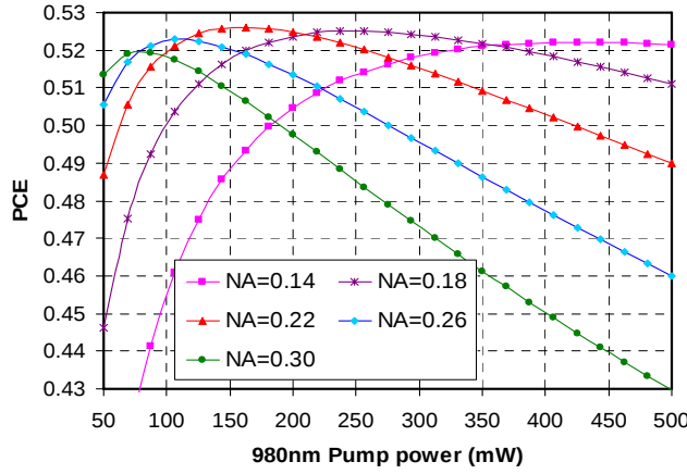
Fig. 1 PCE vs. pump power for different fiber NAs
