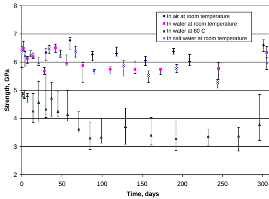
Figure 1: Acrylate fiber aging behavior in water
