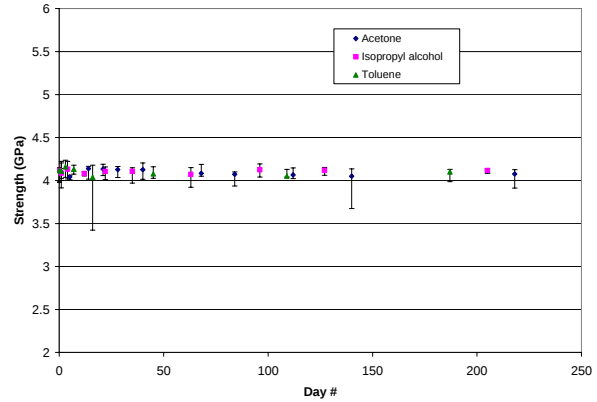
Figure 8: Aging behavior of carbon-polyimide fiber in chemicals
