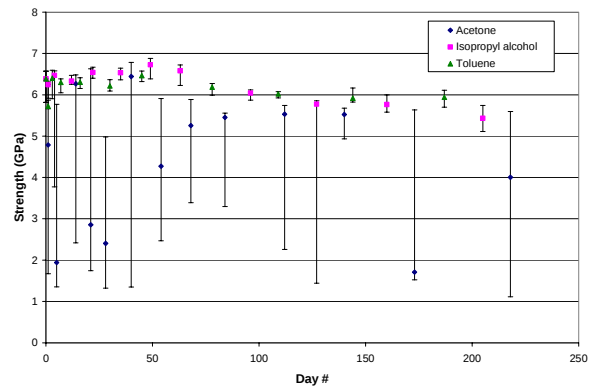
Figure 2: Acrylate fiber aging behavior in chemicals
