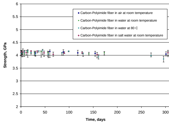
Figure 7: Aging behavior of carbon-polyimide fiber in water
