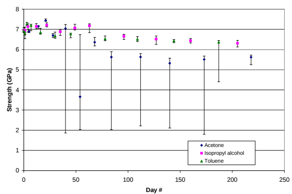
Figure 6: Aging behavior of polyimide fiber in chemicals
