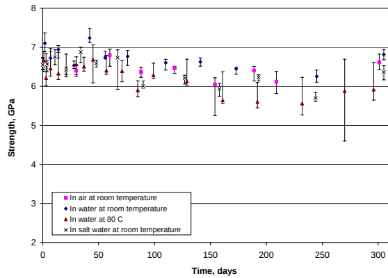
Figure 3: HCS fiber aging behavior in water
