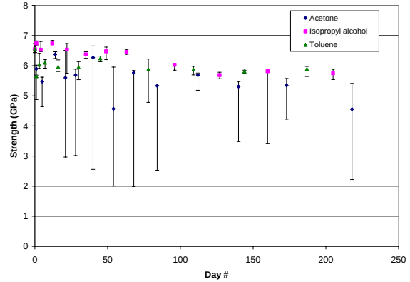
Figure 4: HCS fiber aging behavior in chemicals
