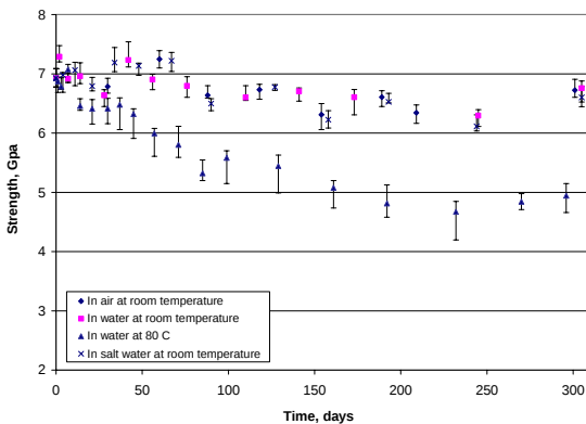
Figure 5: Aging behavior of polyimide fiber in water
