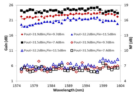
Figure 3: Net gain and NF from the clad-pumped L-band EDFA
