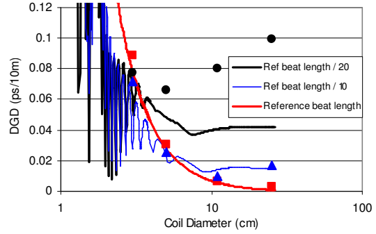
Fig. 4: Simulations of DGD vs. bending diameter for different values of intrinsic beat length along with data from fig. 3. When the beat length decreases, it interferes with the spin period resulting in a quickly varying PMD. Such extreme variations would be very difficult to resolve experimentally, but show that PMD is very difficult to predict when bending high PMD fibers.
