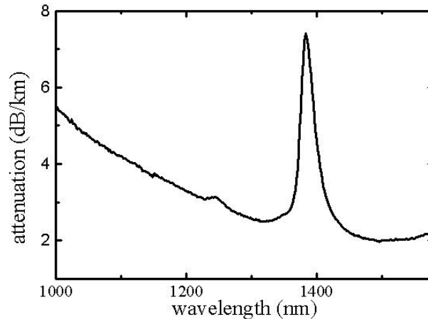
Fig. 3. Attenuation spectrum of the single-mode fiber displayed in Figure 1a.
